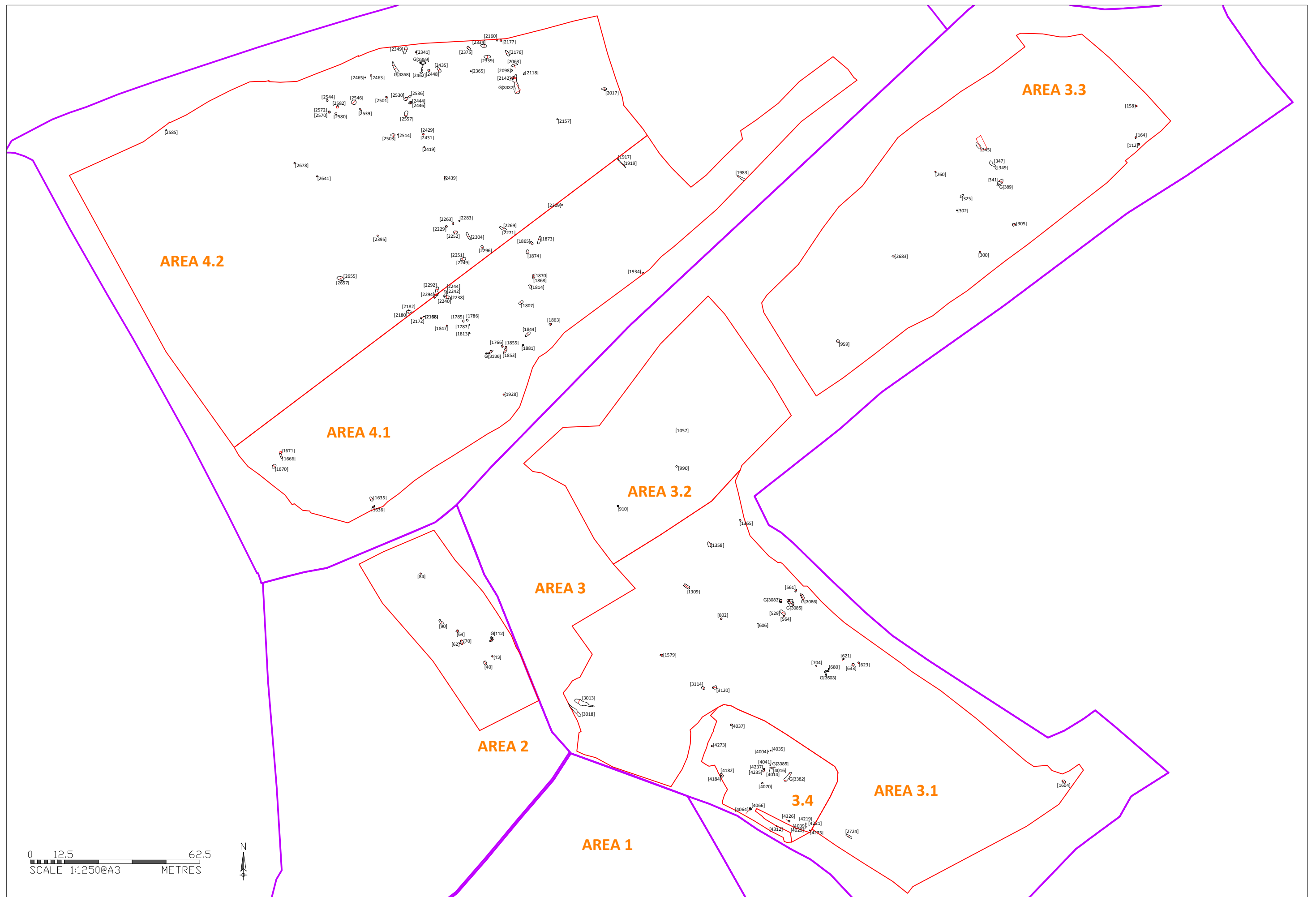
Figure 16: Unphased features
